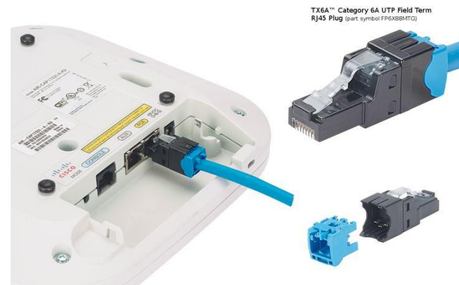
TX6A™ Category 6A UTP Field Term RJ45 Plug (part symbol FP6X88MTG)
